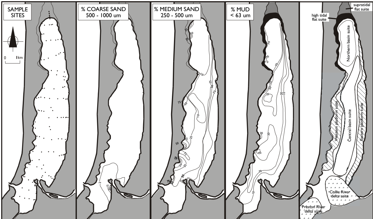
Figure 4. Maps showing sampling sites and the distribution of the coarse sand, medium sand, and mud in Leschenault Inlet (after Wurm & Semeniuk 2000). Final map shows sediment suites (or facies) based on grain sizes and geomorphic setting.
