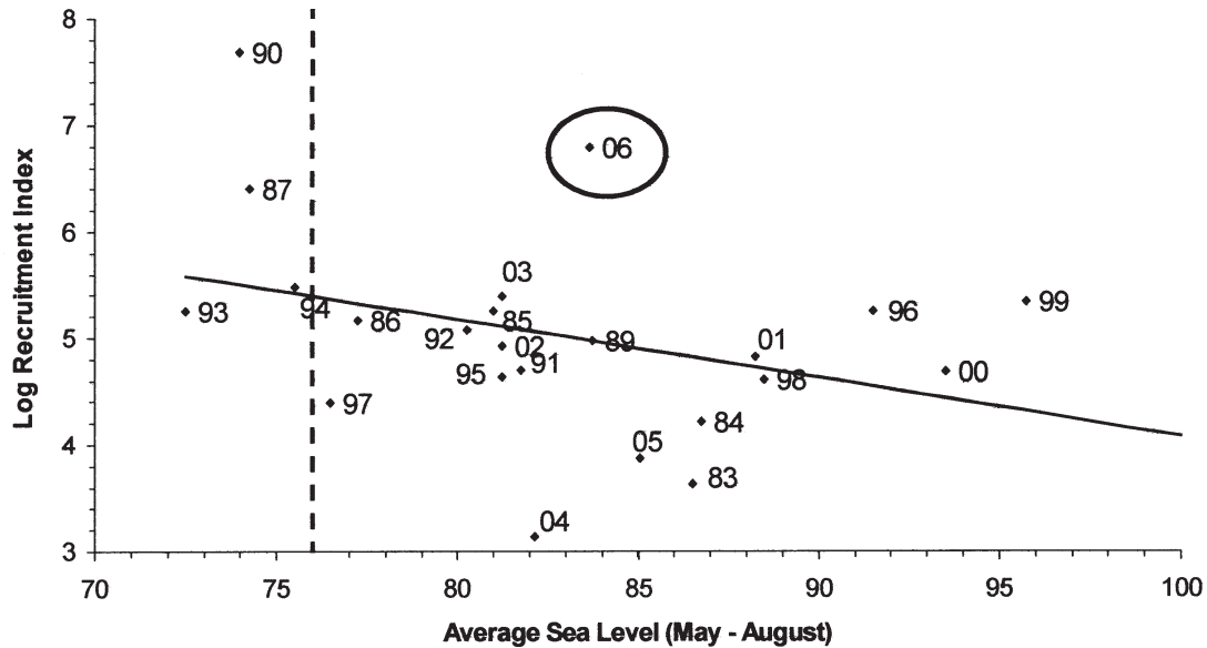
Figure 6. Correlation ( \log(\text{Recruitment}) = 9.6 - 0.06\text{FSL} , R^2 = 0.14 ) between recruitment index in the Shark Bay scallop fishery (northern ground) and Leeuwin Current strength (FSL) between May and August (1983–2006). Dashed line indicates low average FSL conditions where some recruitment was observed to be high. Note 2006 is highlighted as a year with higher recruitment even though FSL was average.
