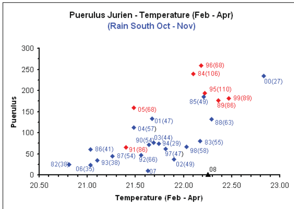
Figure 3. Relationship between the annual puerulus settlement (mean number per collector) at Jurien, and sea surface temperature, at two levels of rainfall (red data points >, and blue data points < than 80 mm, an index of the strength of westerly winds) in October–November, off the lower west coast of Western Australia (updated from Caputi et al. 1996). The predicted level of puerulus settlement for 2008 is presented. The multiple correlation is 0.82 ( p < 0.001 ) for 1982–2006 data.
