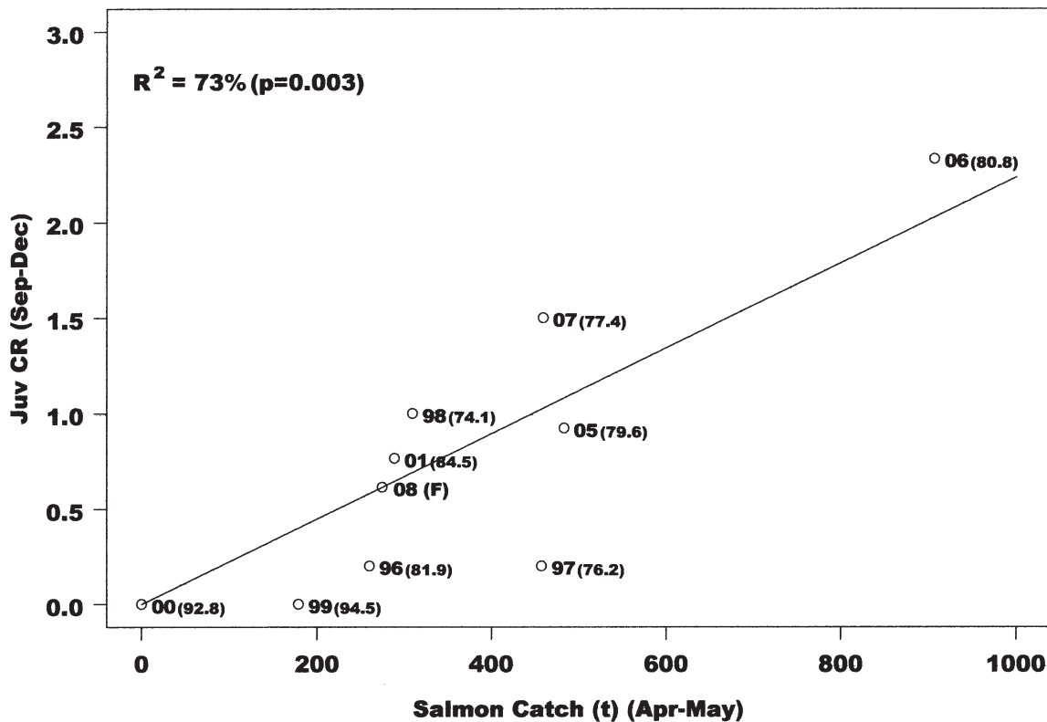
Figure 11. The relationship ( Juv\ CR = -0.2123 + 2.6414 \times 10^{-3} \text{ catch (t)} ) between the annual index of the West Coast Australian Salmon breeding stock (April to May catch), and the annual index of juvenile (0+ yr class) recruitment (measured between September and December of the same year). Mean Fremantle sea level (February to May) is presented in parenthesis after each annual data point. Note that recruitment data were not collected between 2002 and 2004. Recruitment forecast for 2008 is also presented (F).
