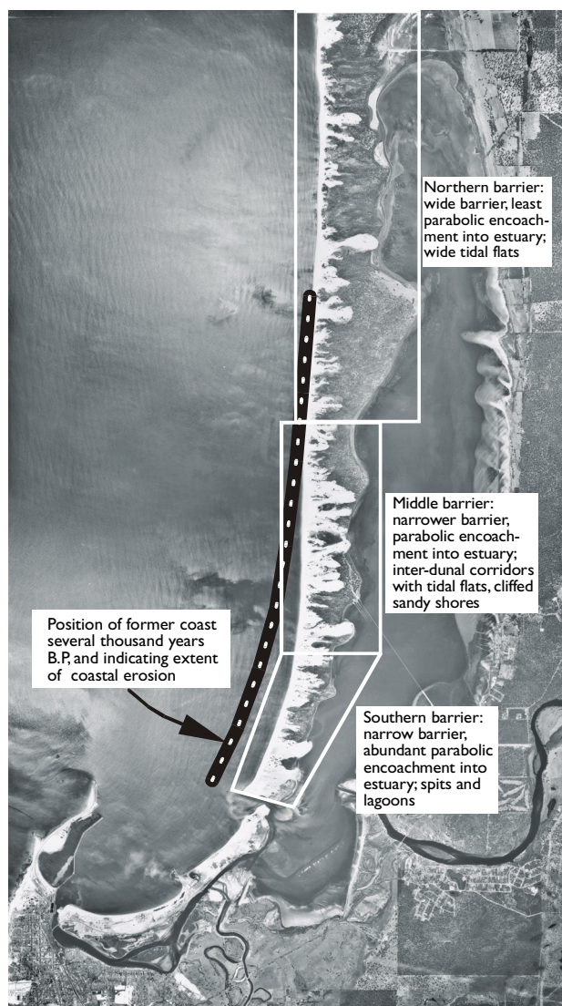
Figure 34. The various sectors along the Leschenault Peninsula showing south to north variation in erosion of the barrier, and its effect on parabolic dunes encroaching into the estuary.
