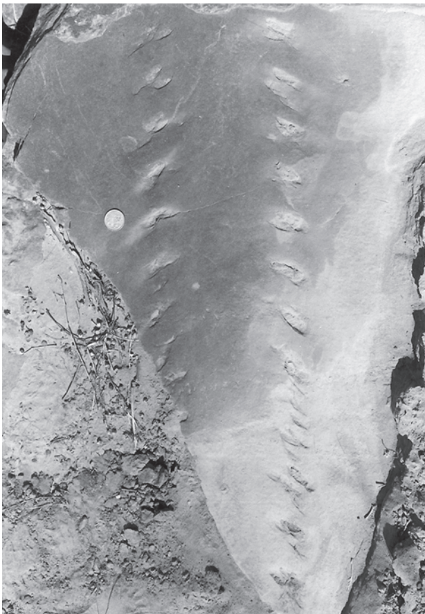
Figure 9 Large Diplichnites trackway about 25 cm in width. Field specimen, bottom of the gorge, eastern side of The Loop; FA2. Diameter of coin 28.5 mm.
